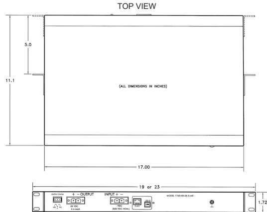
REAR PANEL VIEW OF M5 VERSION
