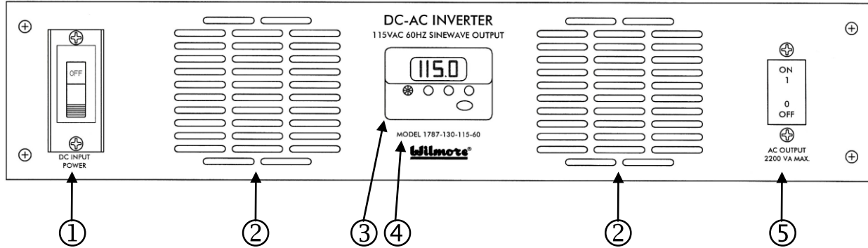
FIGURE 1. FRONT PANEL
