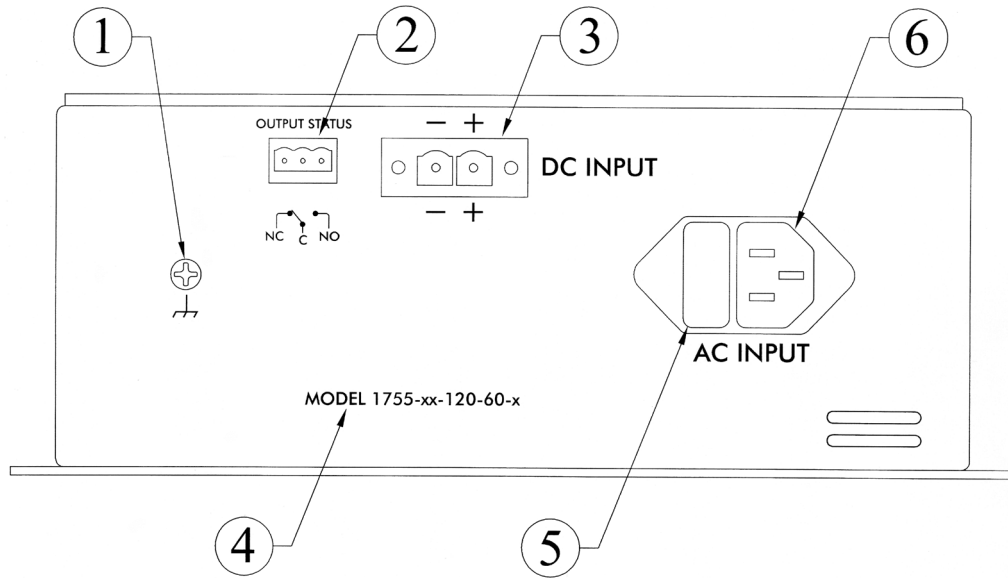
FIGURE 2. REAR PANEL
