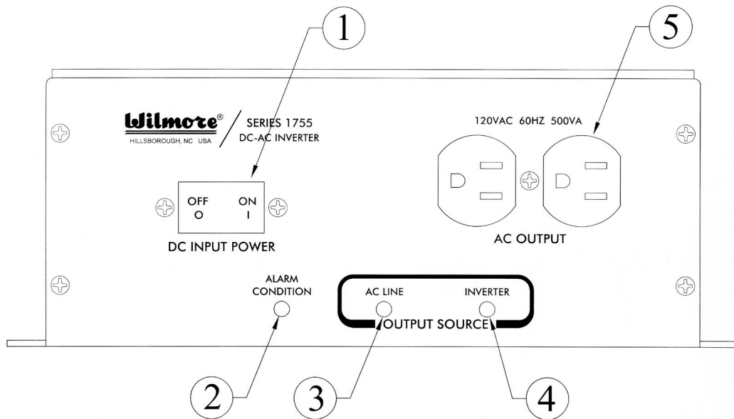
FIGURE 1. FRONT PANEL
