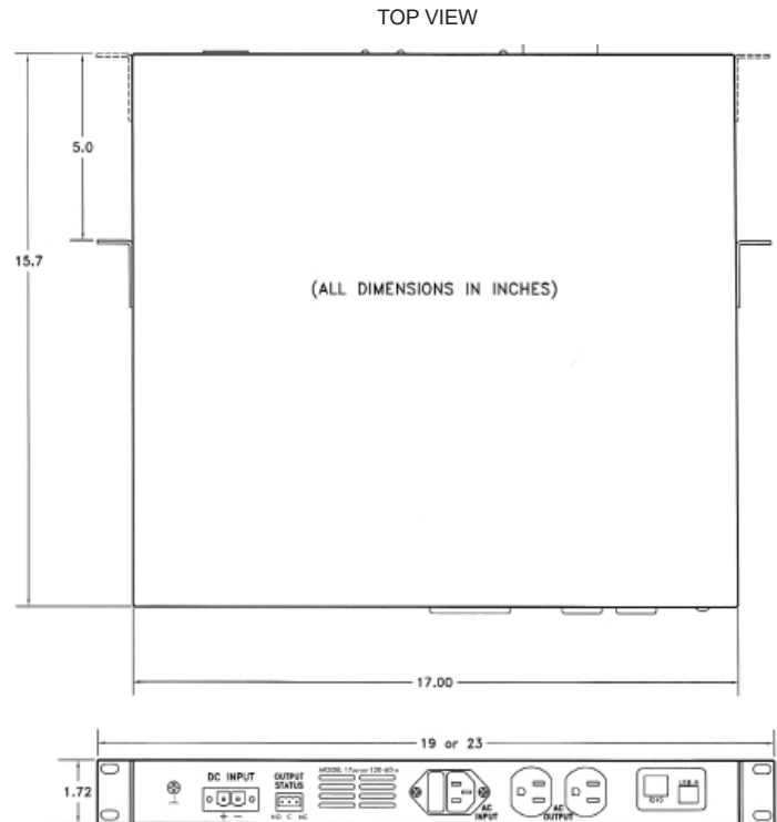
REAR VIEW OF MODEL 1786 U AND L VERSIONS
