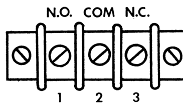
FIGURE 2. AUXILIARY CONTACT TERMINAL BLOCK
