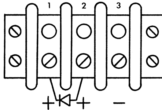
FIGURE 1. OUTPUT TERMINAL BLOCK
