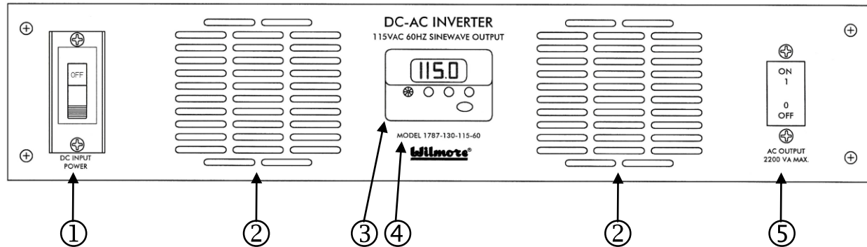
FIGURE 1. FRONT PANEL
