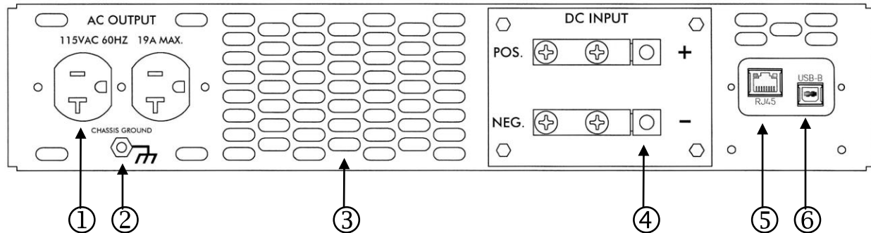
FIGURE 2. REAR PANEL (cover panel removed)
