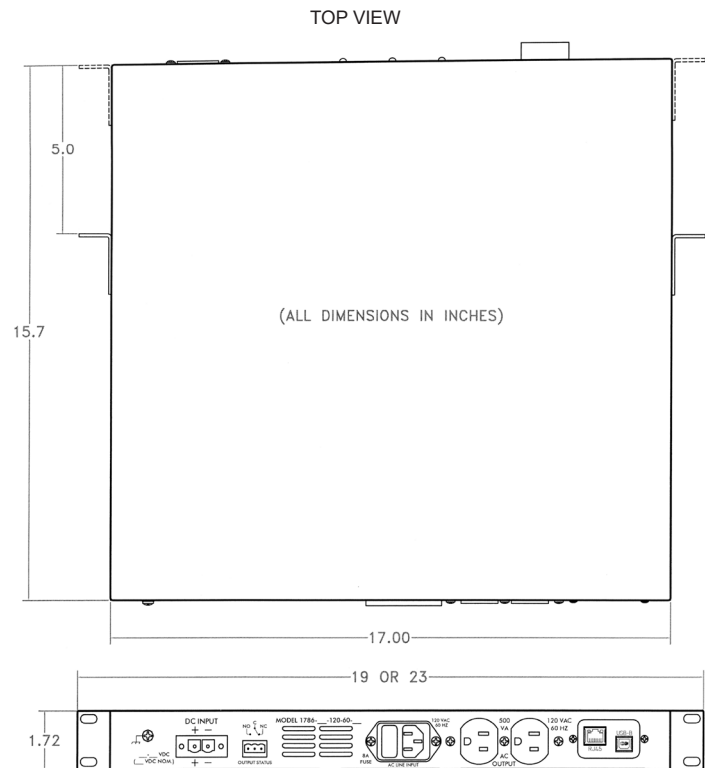
REAR VIEW OF MODEL 1786 U AND L VERSIONS
