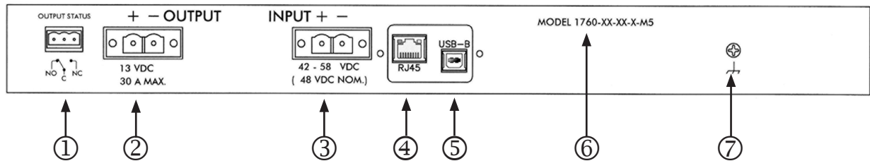
FIGURE 2. REAR PANEL (shown without plugs attached)
