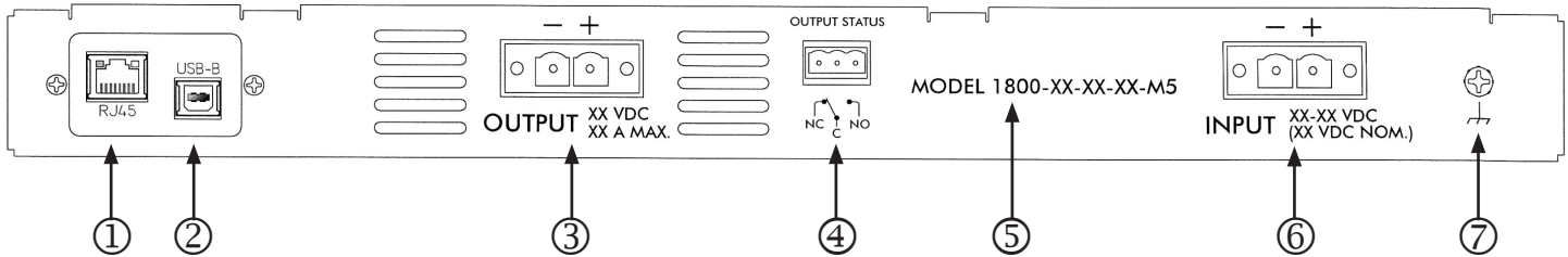
FIGURE 2. REAR PANEL (shown without plugs)
